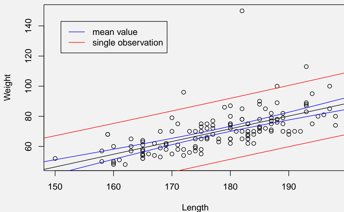
two types of 95% prediction intervals
