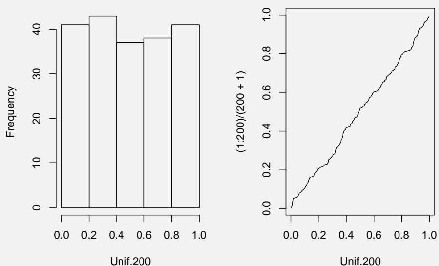
Histogram of Unif.200
